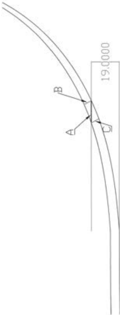
Diagram 19 mm Dimension
